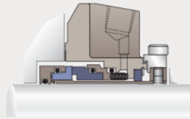
Single pusher
